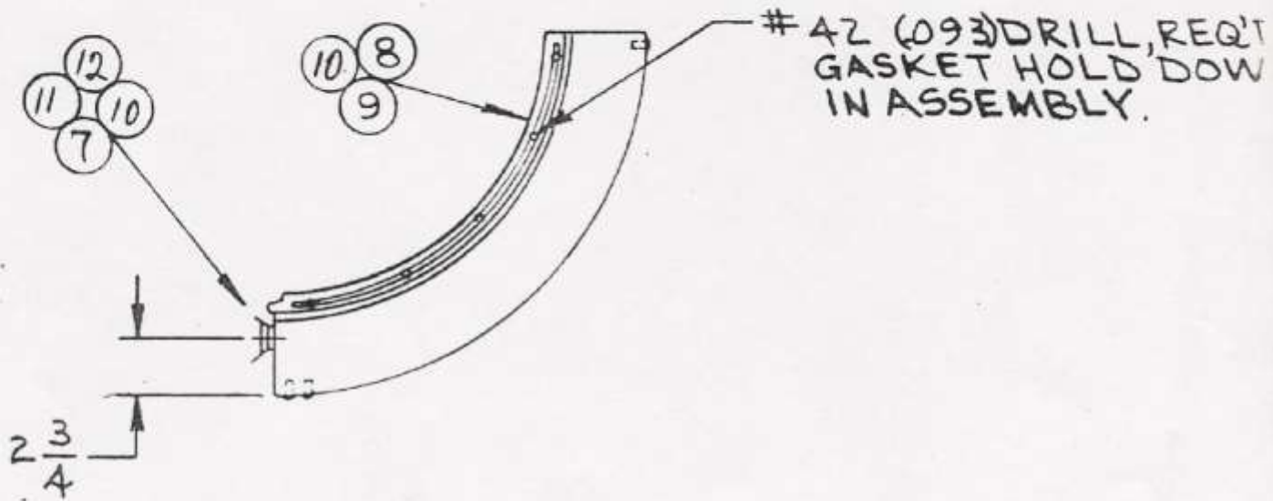
GASKET LOCATION-LOWER DOOR
