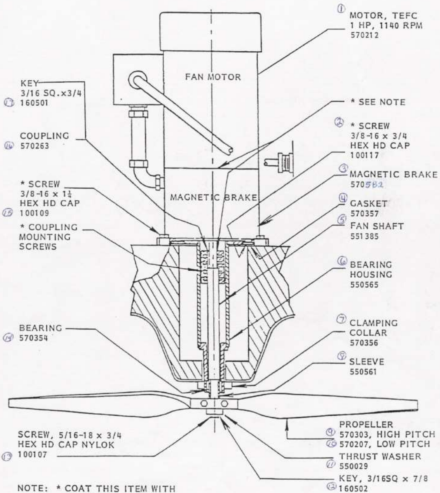
FIXED SPEED FAN ASSEMBLY (with brake) D30-550568
